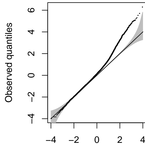
Expected quantiles
